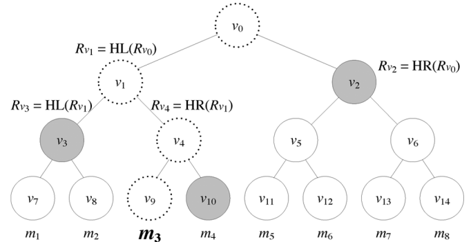
Fig. 1. Illustration of a binary tree used to manage RGK. Im_3 for m_3 located at v_9 should include all of the secret values in the tree except Rv_0 , Rv_1 , Rv_4 , and Rv_9 . As a result, Im_3 contains Rv_2 , Rv_3 , and Rv_{10} . The rest of the secret values are derived.
