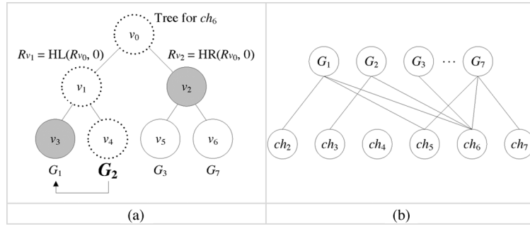
Fig. 2. (a) Illustration of a binary tree for the common channel, ch_6 , when a member m_k changes the group from G_2 to G_1 . Rv_3 , the restricted secret value of G_1 , should be changed because m_k knows Rv_3 . (b) ch_2 , ch_5 , and ch_6 belong to G_1 . ch_3 and ch_6 belong to G_2 . ch_6 is a common channel of G_1 , G_2 , G_3 , and G_7 .
